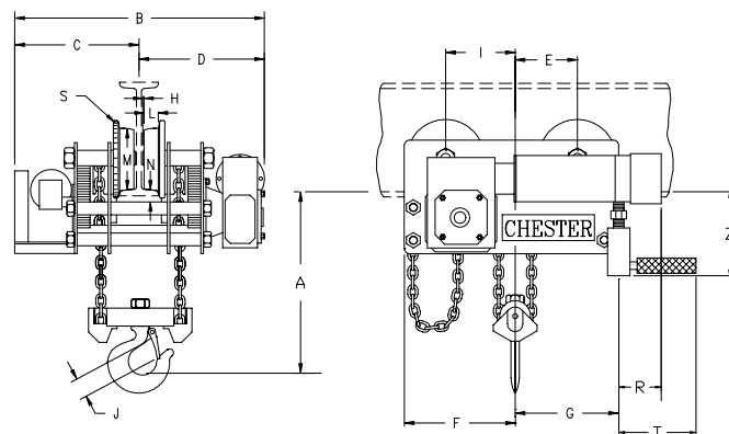
3 & 4 TON PLAIN, GEARED & MOTORIZED
