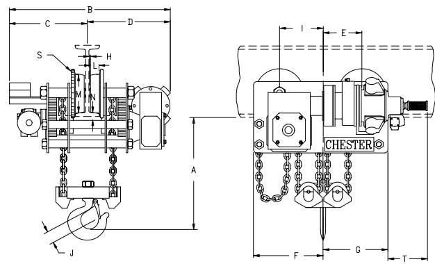
16 TON PLAIN, GEARED & MOTORIZED
